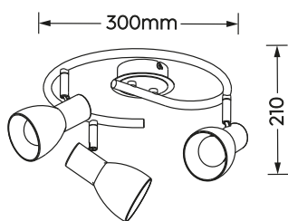
Strahler · Spot incl. 3 x LED E14 3 x 4,9 W / 3 x 470 Lumen 3.000 Kelvin 871090307 871090308
