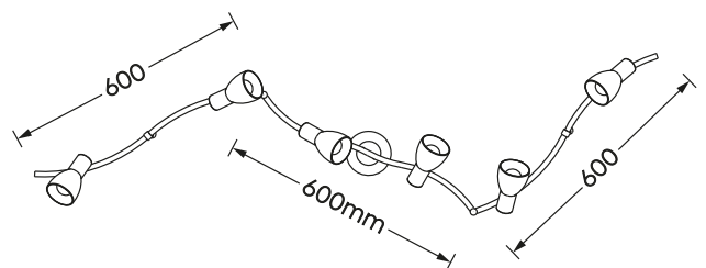
Strahler · Spot incl. 6 x LED E14 6 x 4,9 W / 6 x 470 Lumen 3.000 Kelvin 871010607 871010608
