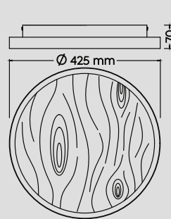
Deckenleuchte · Ceiling lamp incl. SMD-LED 40 W / 4.700 Lumen 3.000 Kelvin 655519130 NEW
